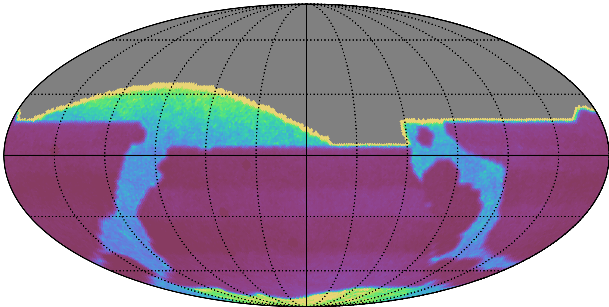
ddf_loaded_half_fl8_v3.4_10yrs : properMotion
