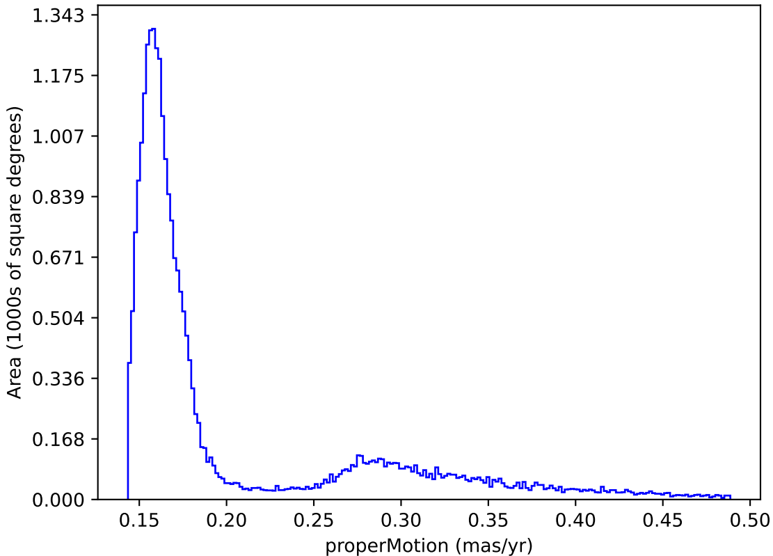
ddf_loaded_half_fl8_v3.4_10yrs : properMotion
