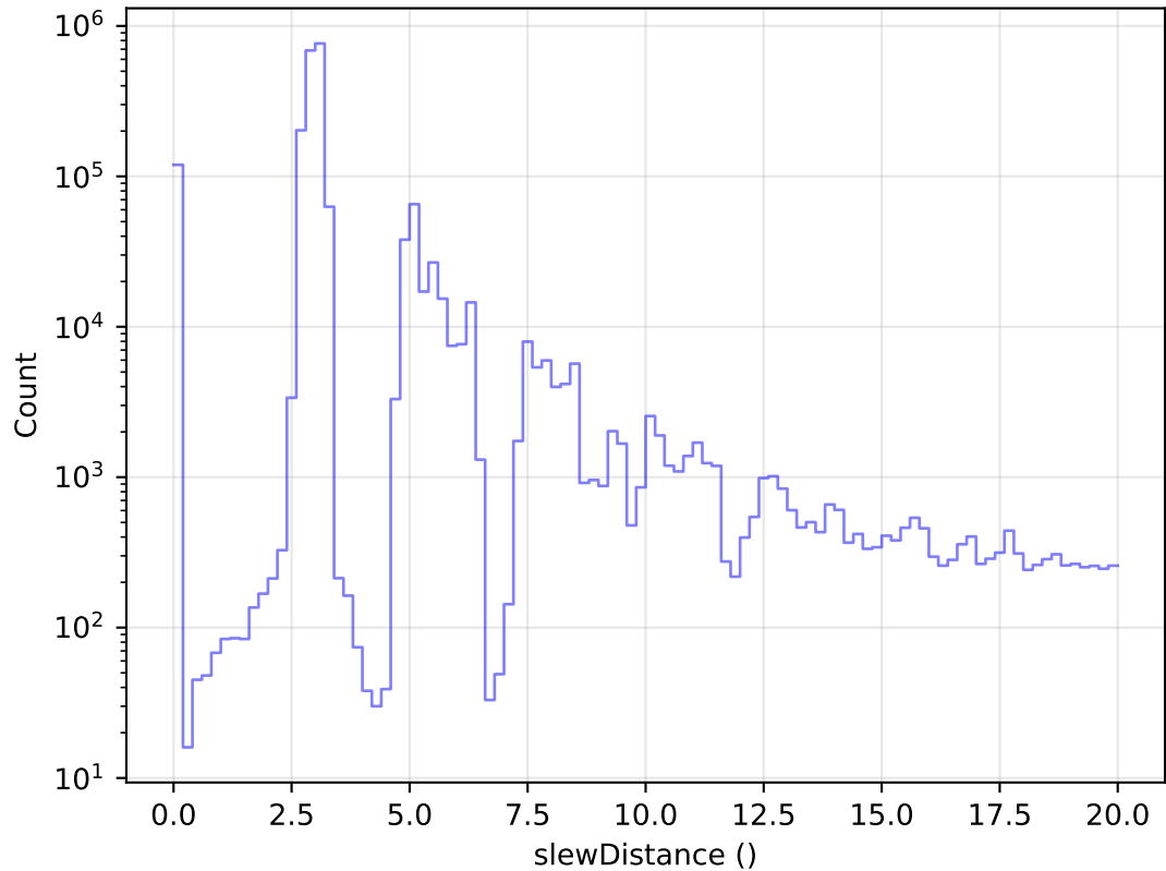
ddf_loaded_half_fl8_v3.4_10yrs All visits: Zoom Slew Distance Histogram
