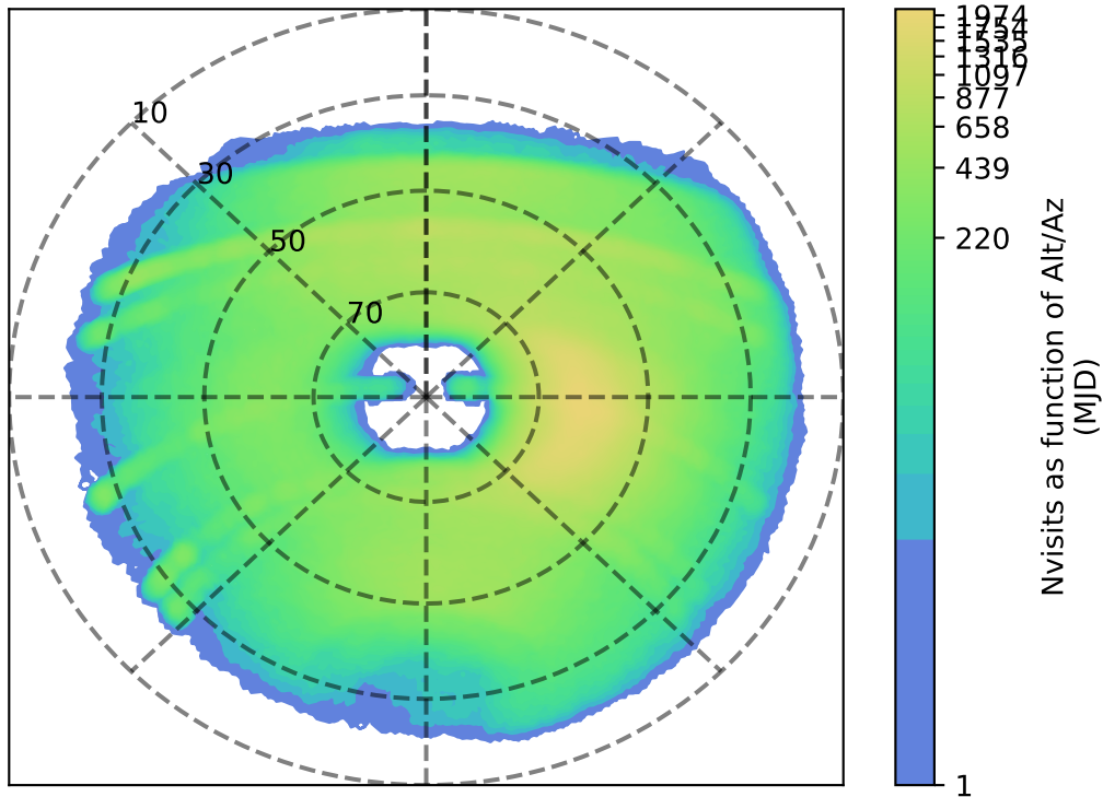
ddf_loaded_half_fl8_v3.4_10yrs y: Nvisits as function of Alt/Az
