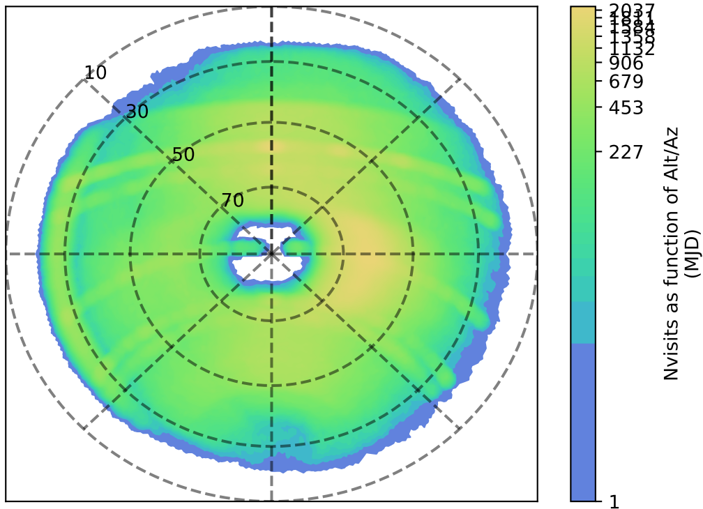
ddf_loaded_half_fl8_v3.4_10yrs r: Nvisits as function of Alt/Az
