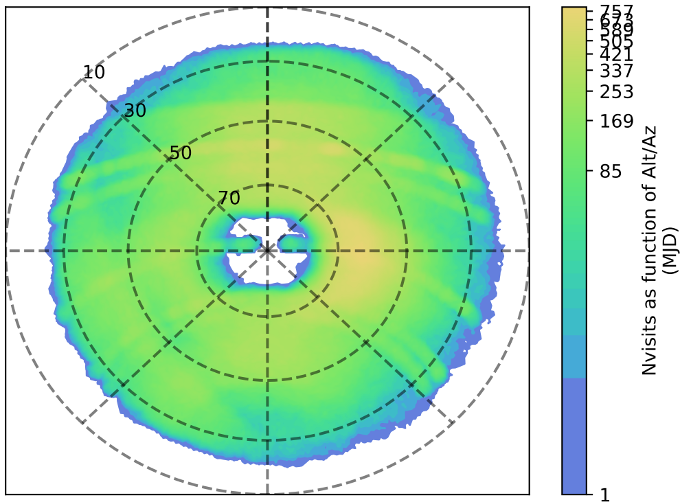
ddf_loaded_half_fl8_v3.4_10yrs g: Nvisits as function of Alt/Az
