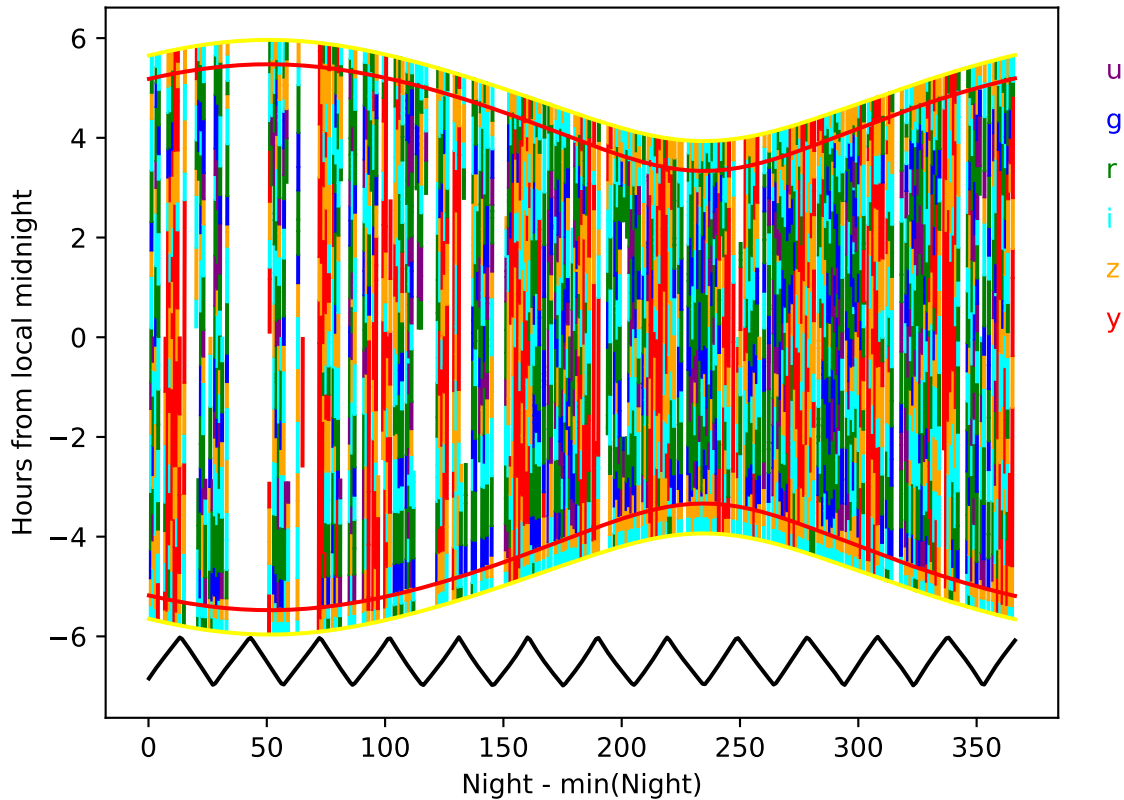
ddf_loaded_half_fl8_v3.4_10yrs year 8-9: Hourglass
