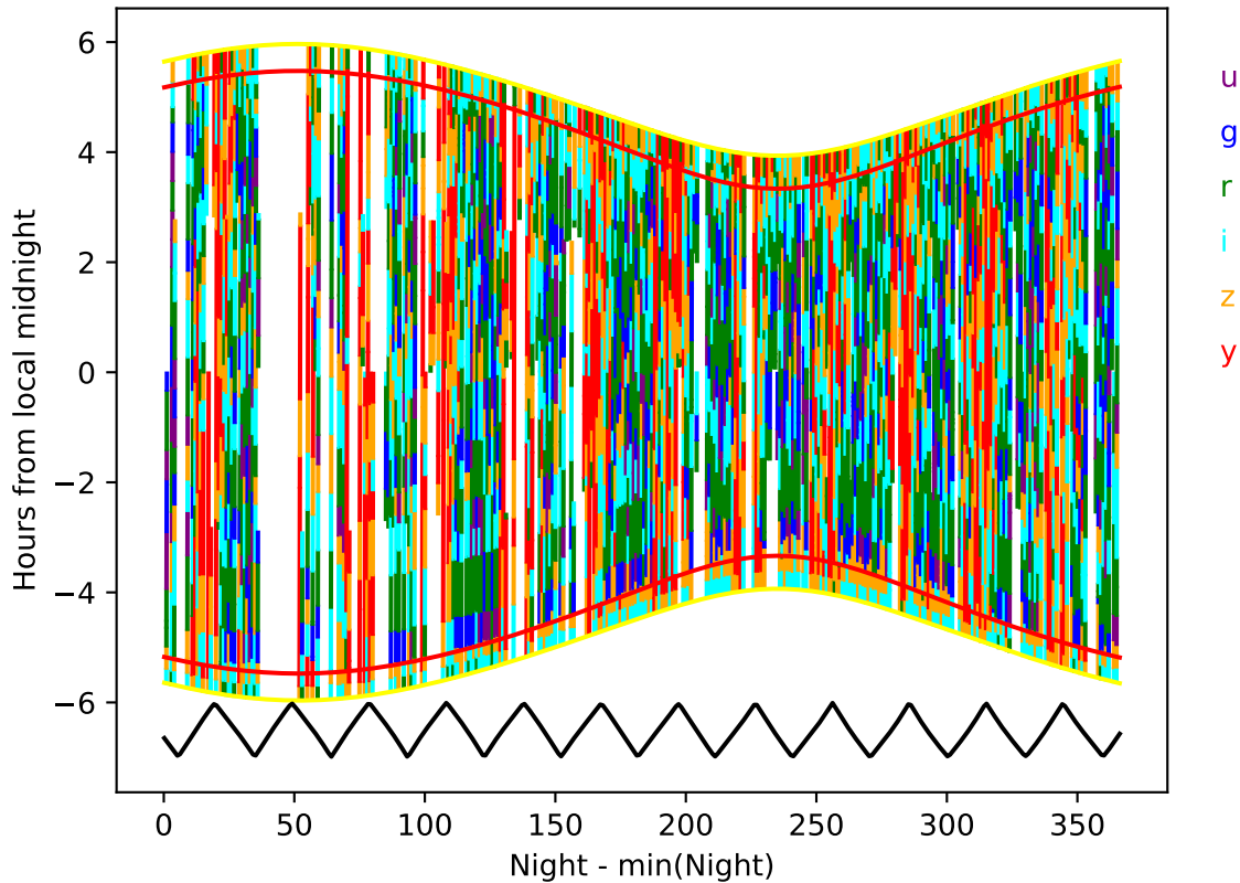
ddf_loaded_half_fl8_v3.4_10yrs year 2-3: Hourglass
