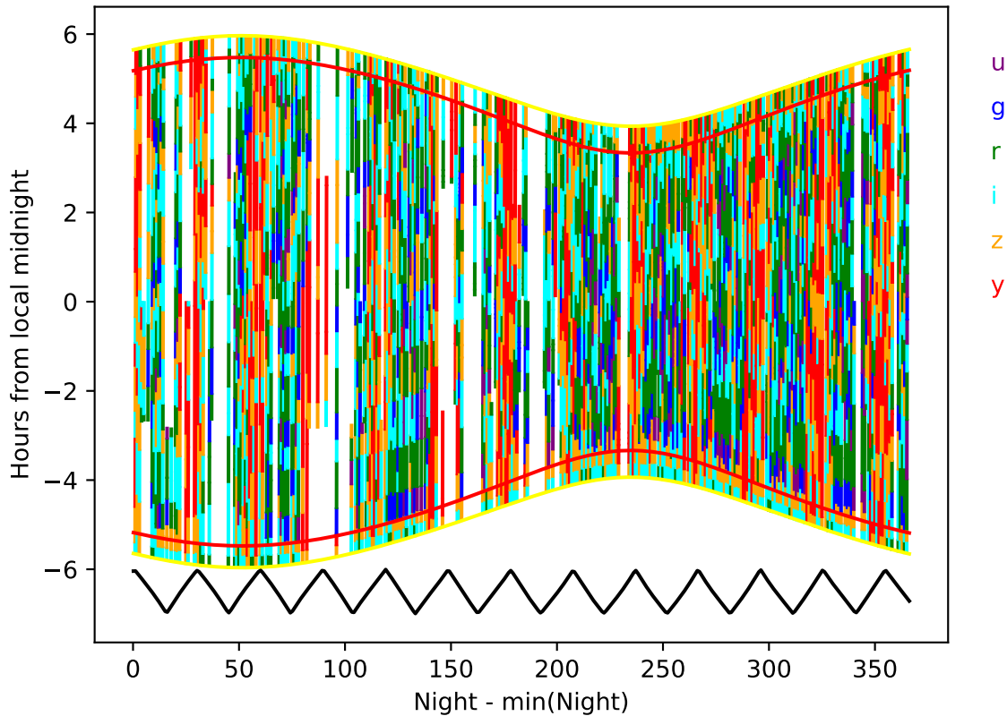
ddf_loaded_half_fl8_v3.4_10yrs year 1-2: Hourglass
