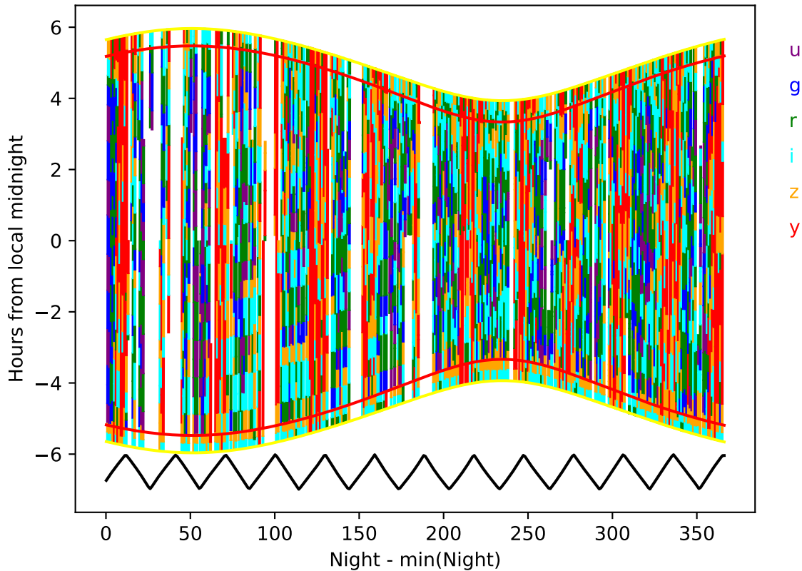
ddf_loaded_half_fl8_v3.4_10yrs year 0-1: Hourglass
