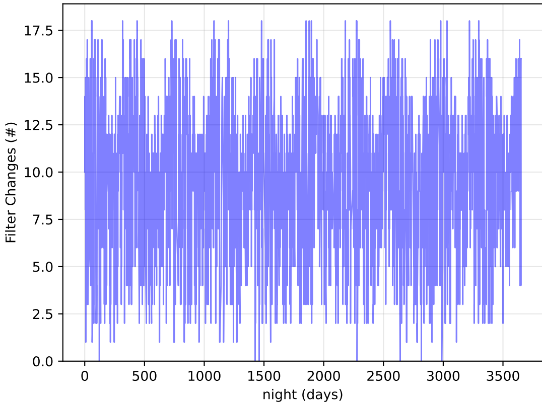
ddf_loaded_half_fl8_v3.4_10yrs : Filter Changes
