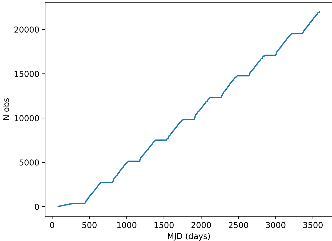
ddf_loaded_half_fl8_v3.4_10yrs note like DD:XMM_LSS%: Cumulative
