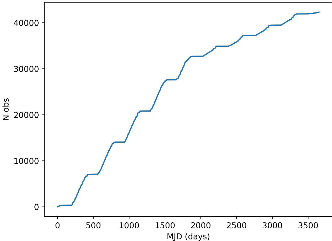
ddf_loaded_half_fl8_v3.4_10yrs note like DD:COSMOS%: Cumulative
