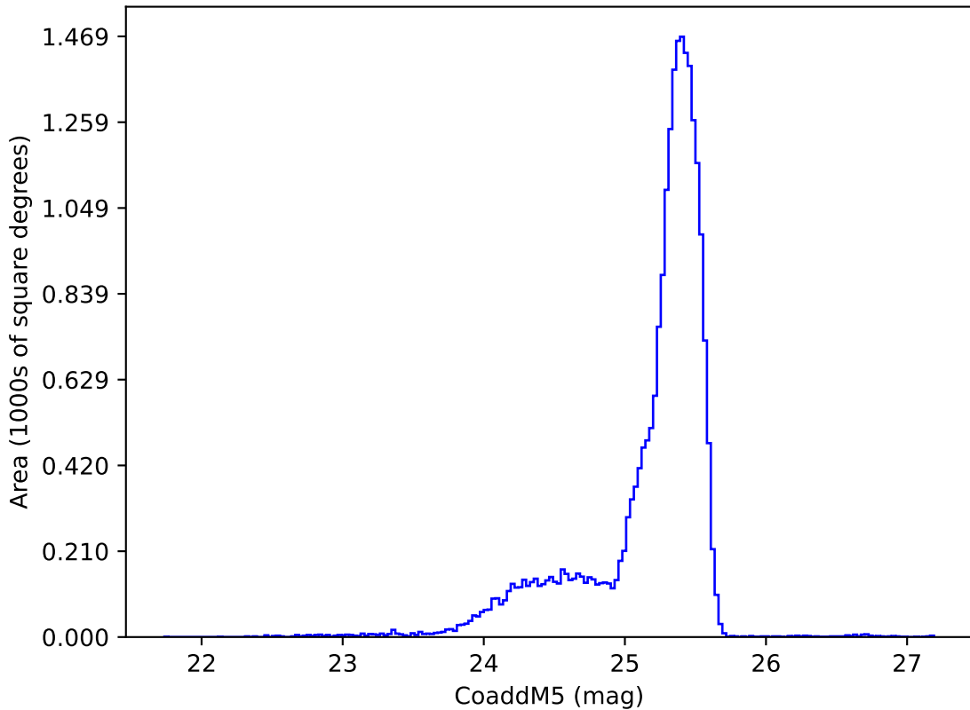
ddf_loaded_half_fl8_v3.4_10yrs u: CoaddM5
