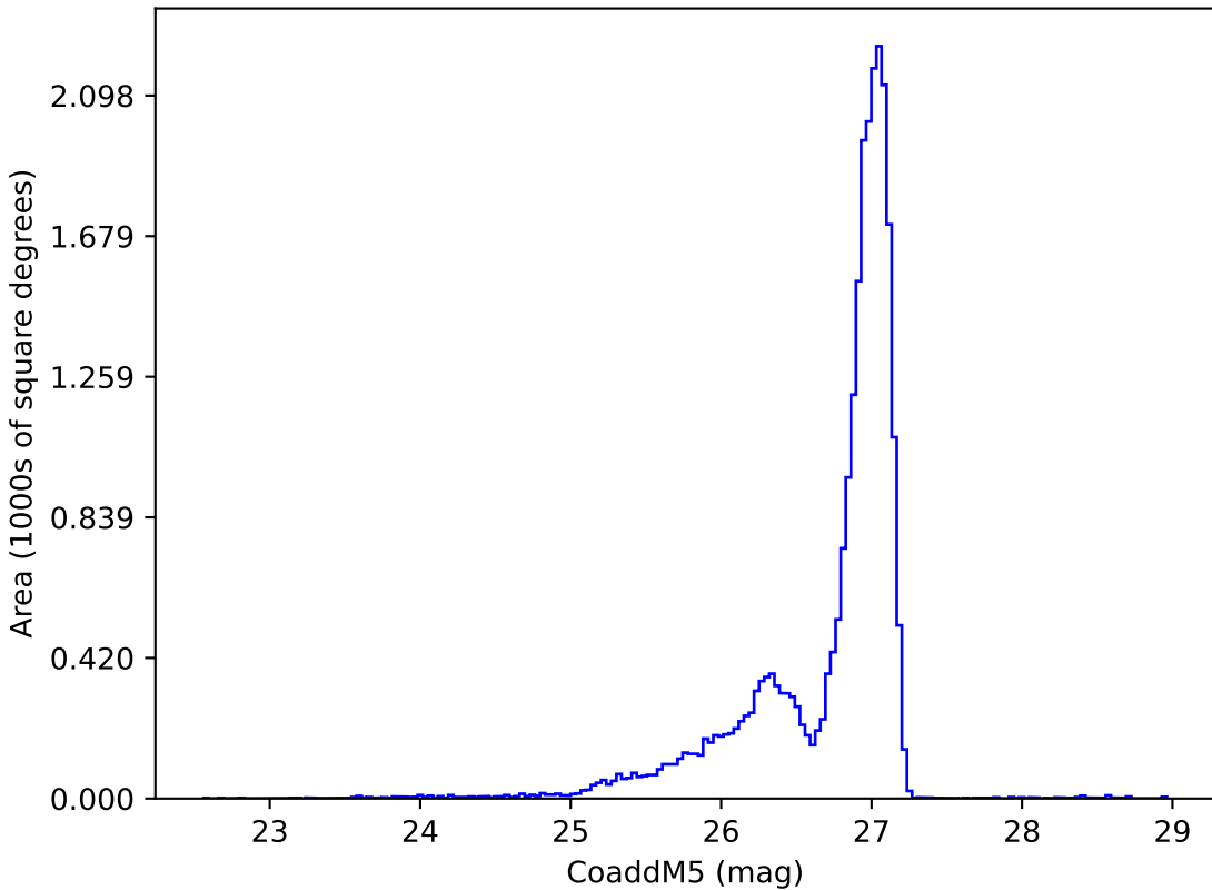
ddf_loaded_half_f18_v3.4_10yrs r: CoaddM5
