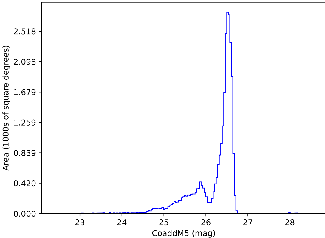
ddf_loaded_half_fl8_v3.4_10yrs i: CoaddM5
