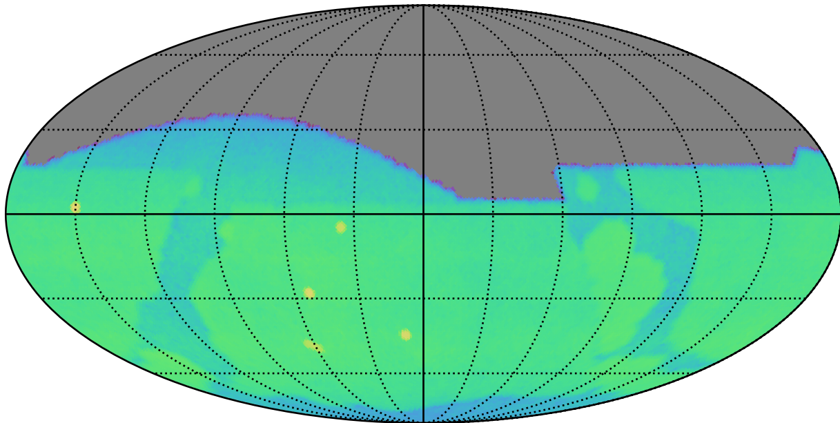
ddf_loaded_half_fl8_v3.4_10yrs g: CoaddM5
