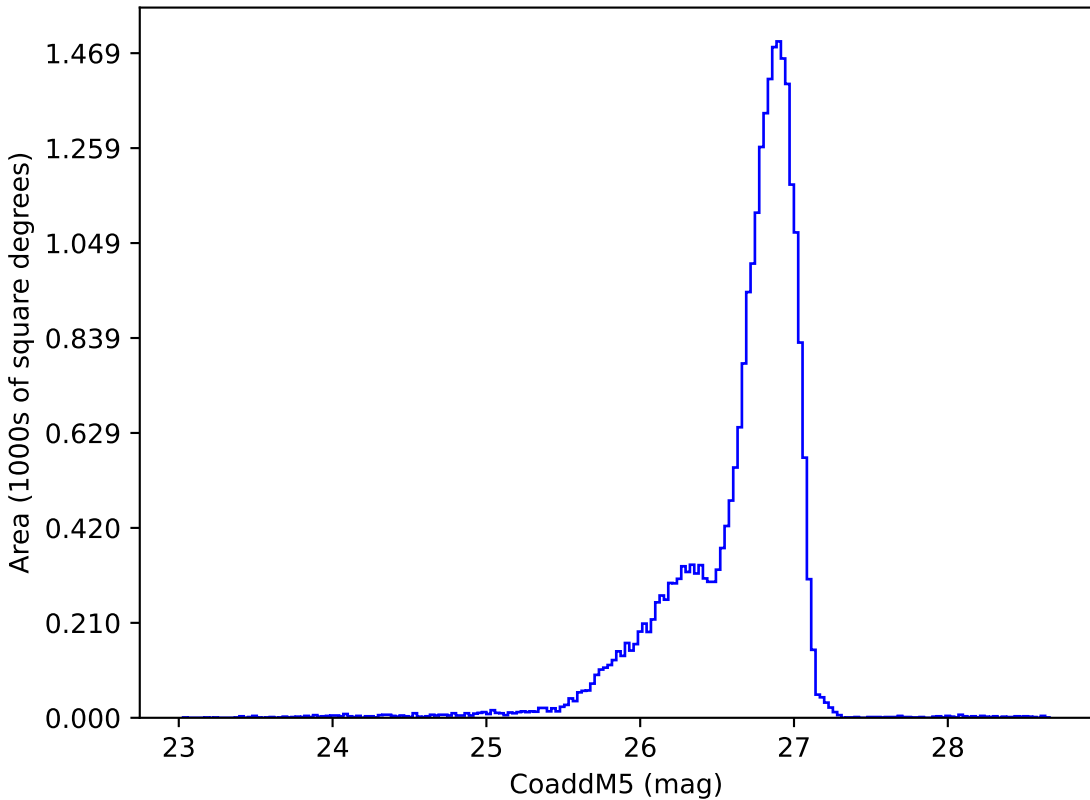
ddf_loaded_half_fl8_v3.4_10yrs g: CoaddM5
