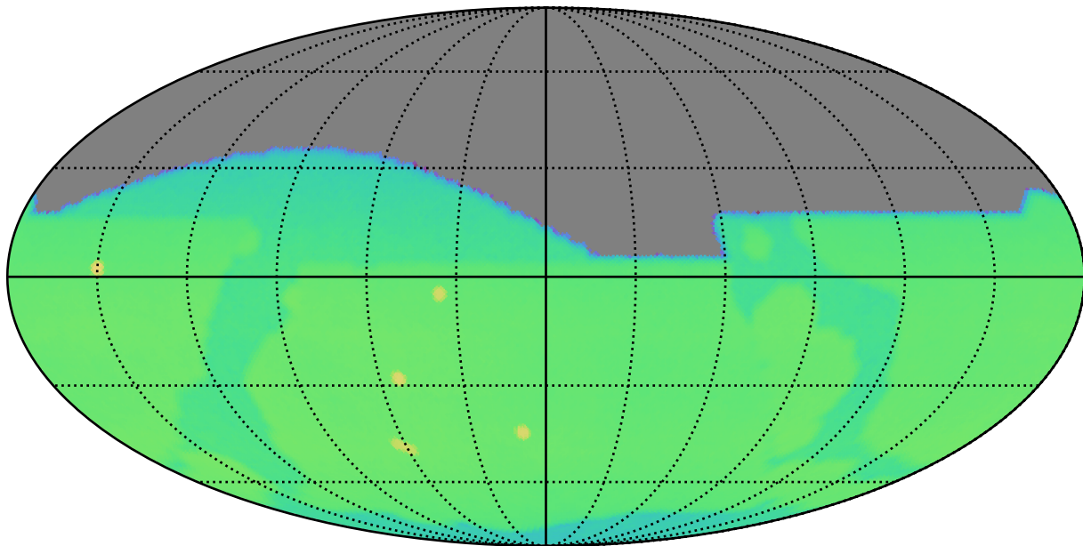
ddf_loaded_half_fl8_v3.4_10yrs : CoaddM5
