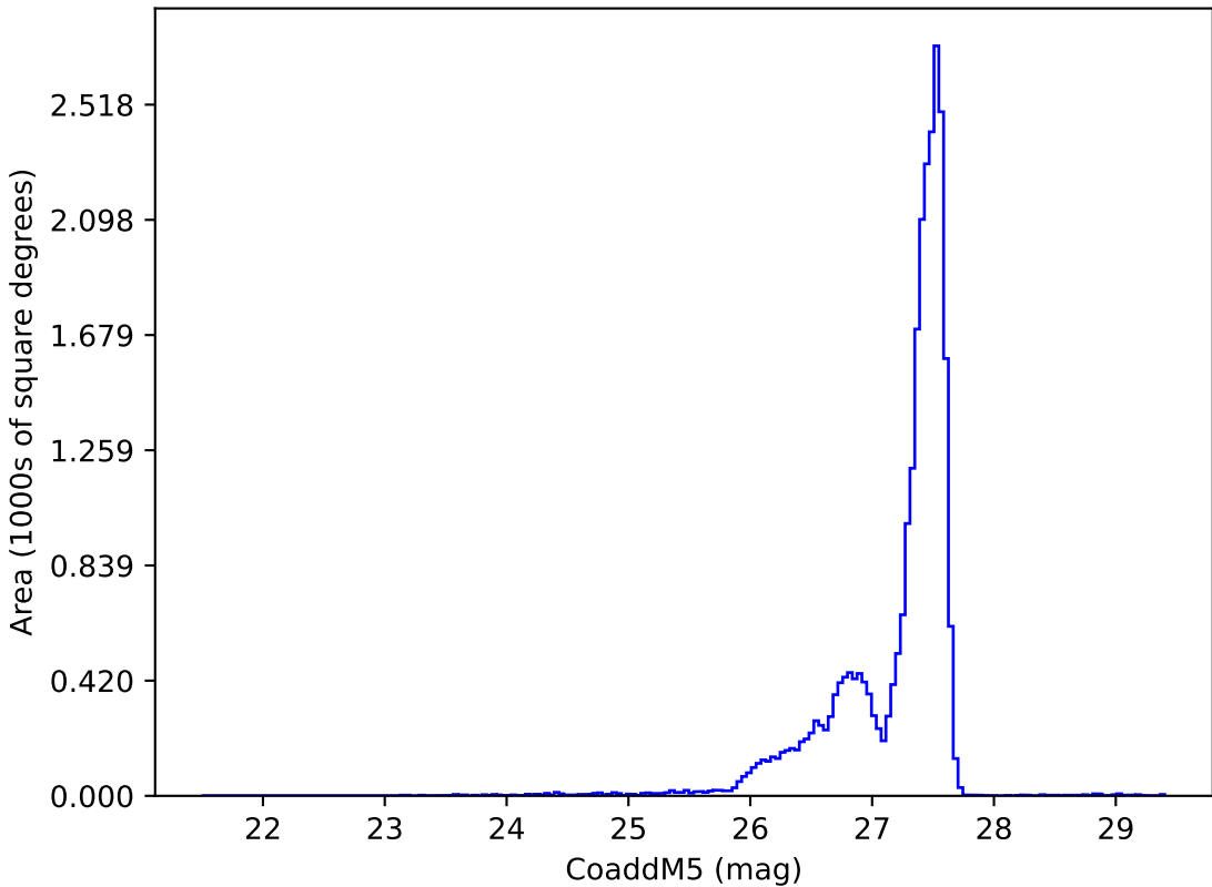
ddf_loaded_half_fl8_v3.4_10yrs : CoaddM5
