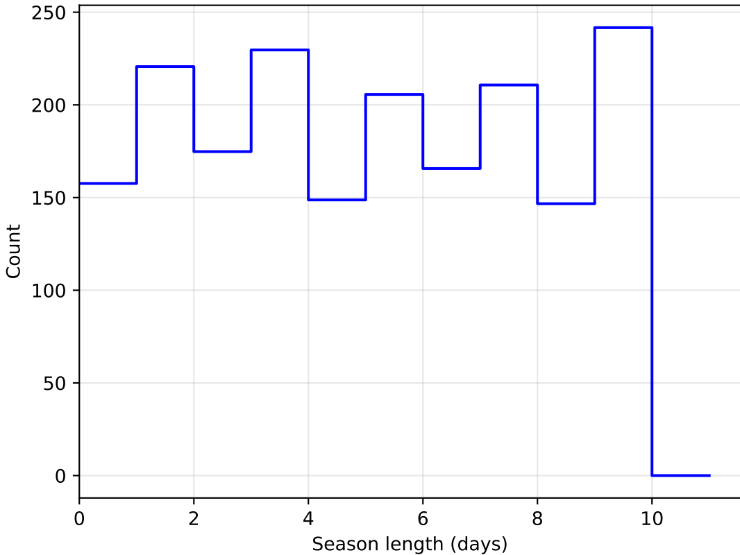
ddf_loaded_half_fl8_v3.4_10yrs DD:WFD all bands: SeasonLength
