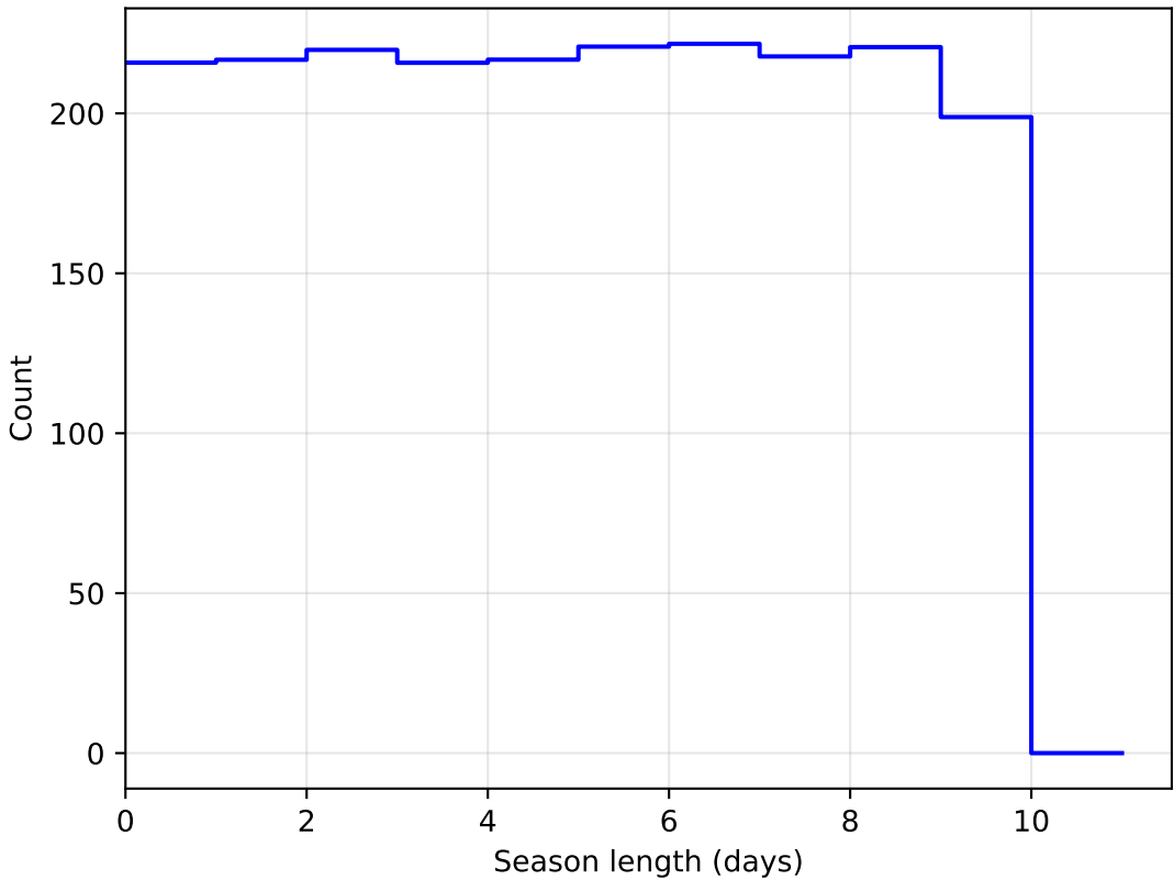
ddf_loaded_half_fl8_v3.4_10yrs DD:EDFS all bands: SeasonLength
