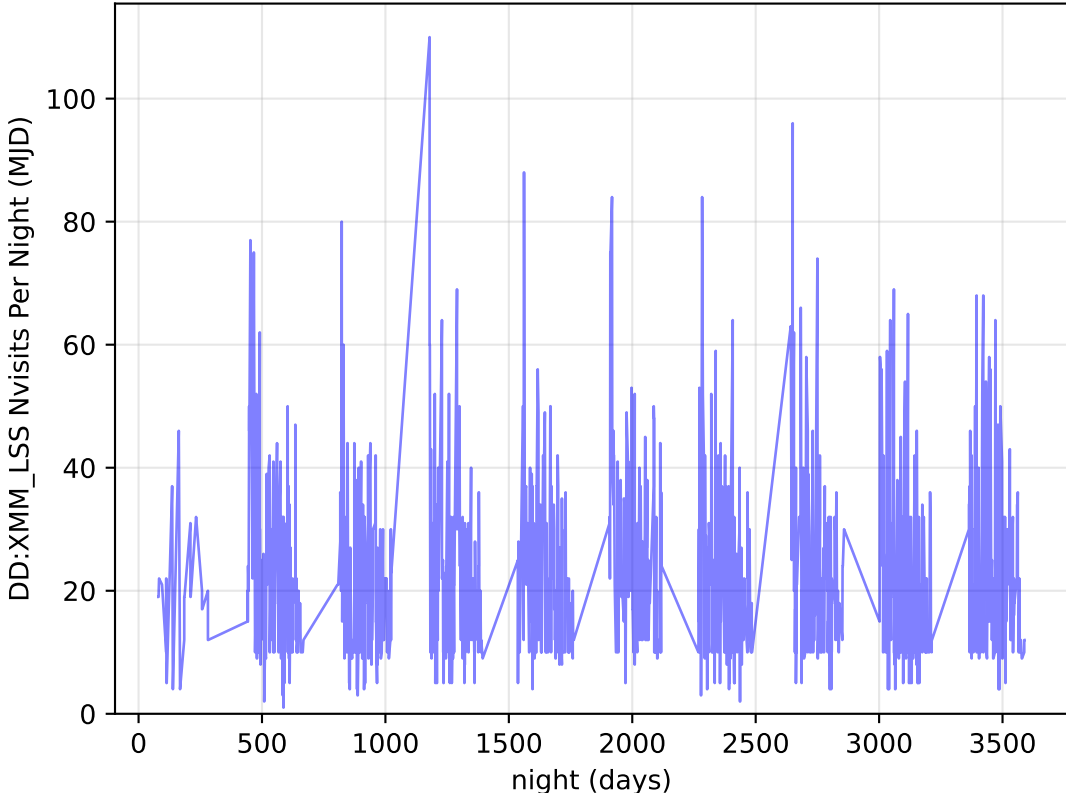
ddf_loaded_half_fl8_v3.4_10yrs all bands: DD:XMM_LSS Nvisits Per Night
