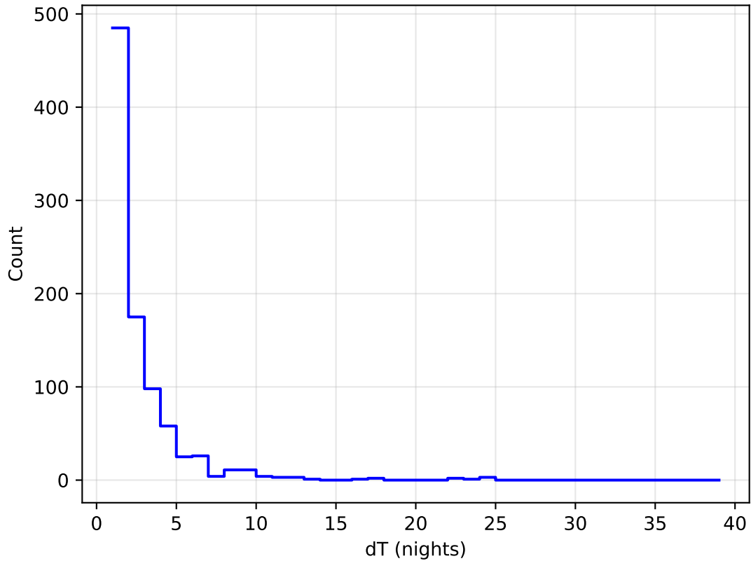
ddf_loaded_half_fl8_v3.4_10yrs all bands: DD:XMM_LSS Delta Nights Histogram
