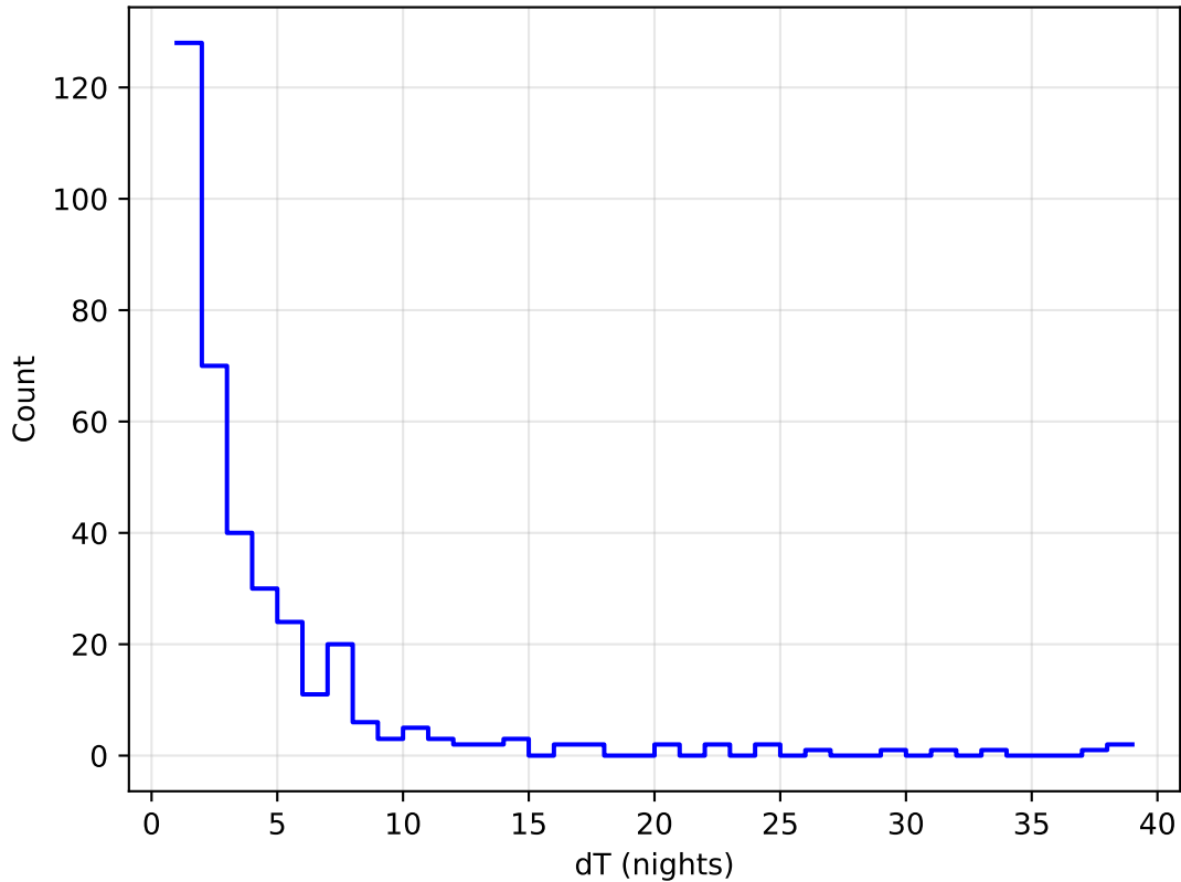
ddf_loaded_half_fl8_v3.4_10yrs all bands: DD:WFD Delta Nights Histogram
