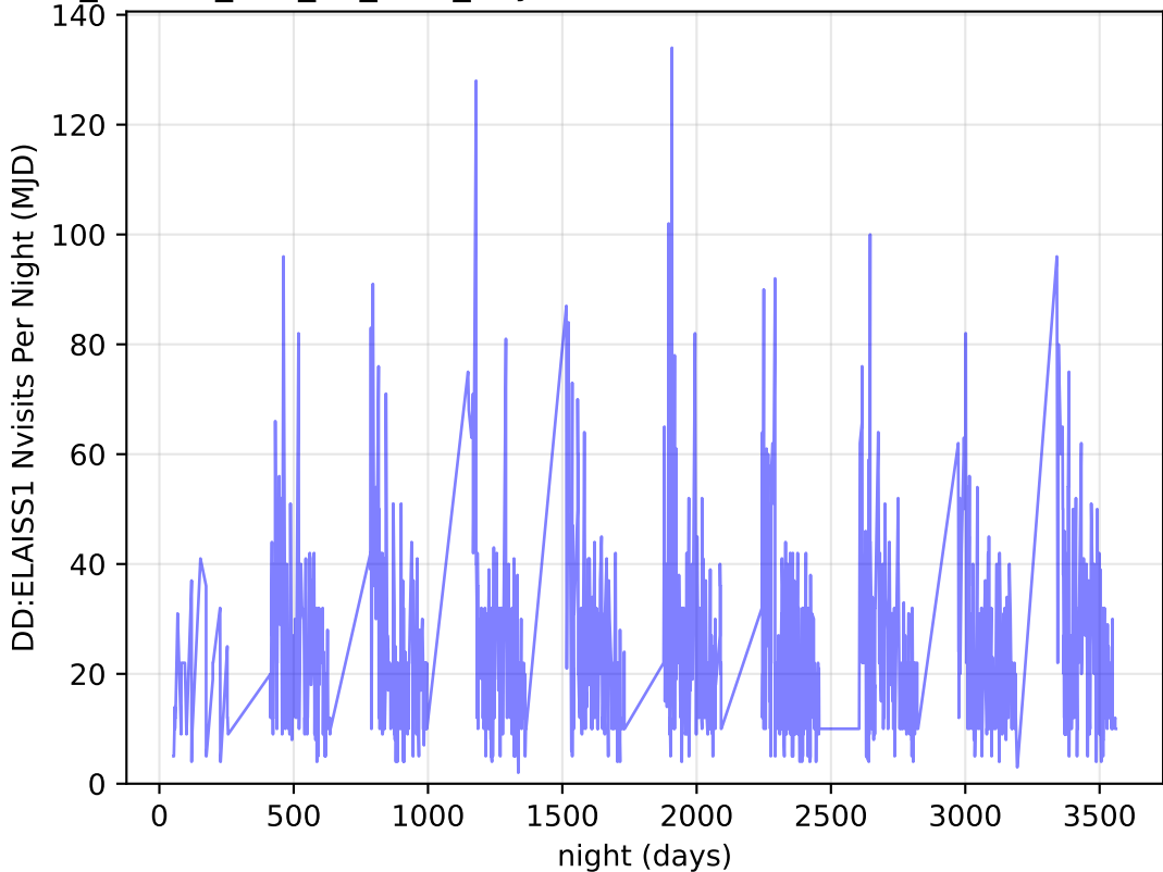
ddf_loaded_half_fl8_v3.4_10yrs all bands: DD:ELAISS1 Nvisits Per Night
