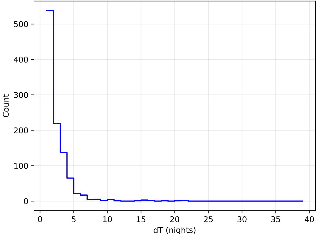
ddf_loaded_half_fl8_v3.4_10yrs all bands: DD:EDFS Delta Nights Histogram
