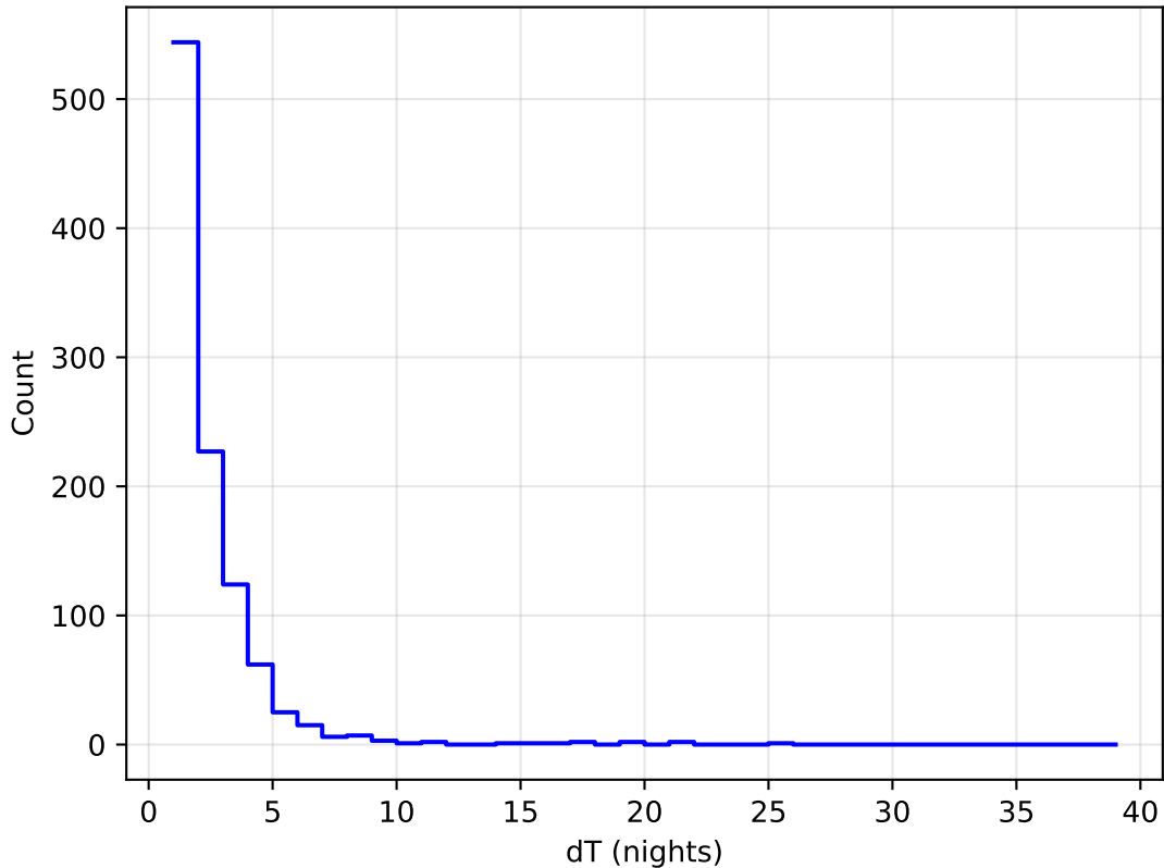
ddf_loaded_half_fl8_v3.4_10yrs all bands: DD:ECDFS Delta Nights Histogram
