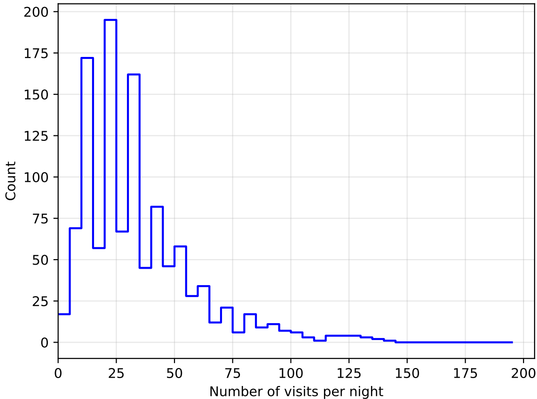
ddf_loaded_half_fl8_v3.4_10yrs all bands: DD: COSMOS NVisitsPerNight
