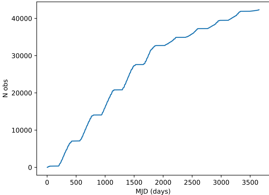
ddf_loaded_half_fl8_v3.4_10yrs all bands: DD:COSMOS Cumulative NVisits
