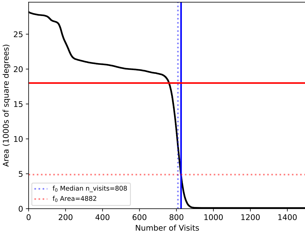
ddf_loaded_half_fl8_v3.3_10yrs : f0
