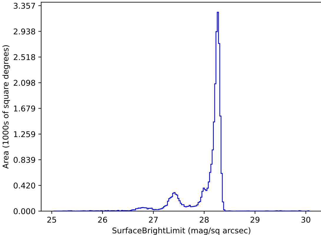
ddf_loaded_half_fl8_v3.3_10yrs y: SurfaceBrightLimit
