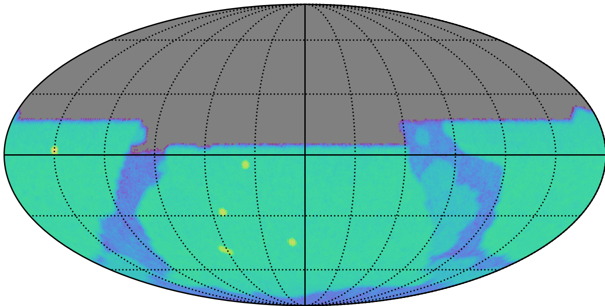
ddf_loaded_half_fl8_v3.3_10yrs u: SurfaceBrightLimit
