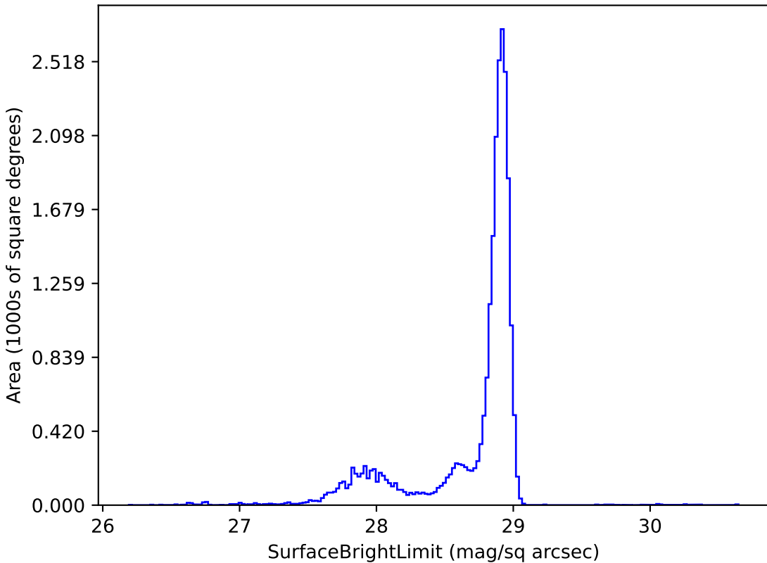
ddf_loaded_half_fl8_v3.3_10yrs u: SurfaceBrightLimit
