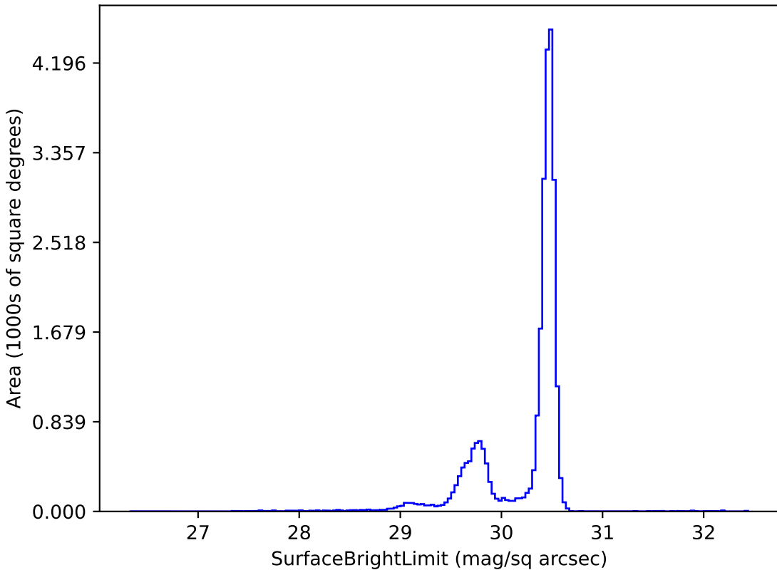
ddf_loaded_half_fl8_v3.3_10yrs r: SurfaceBrightLimit
