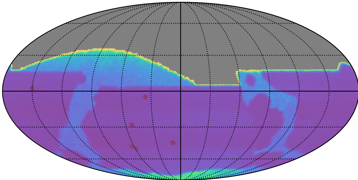
ddf_loaded_half_fl8_v3.3_10yrs : Proper Motion Uncert @ 20.5
