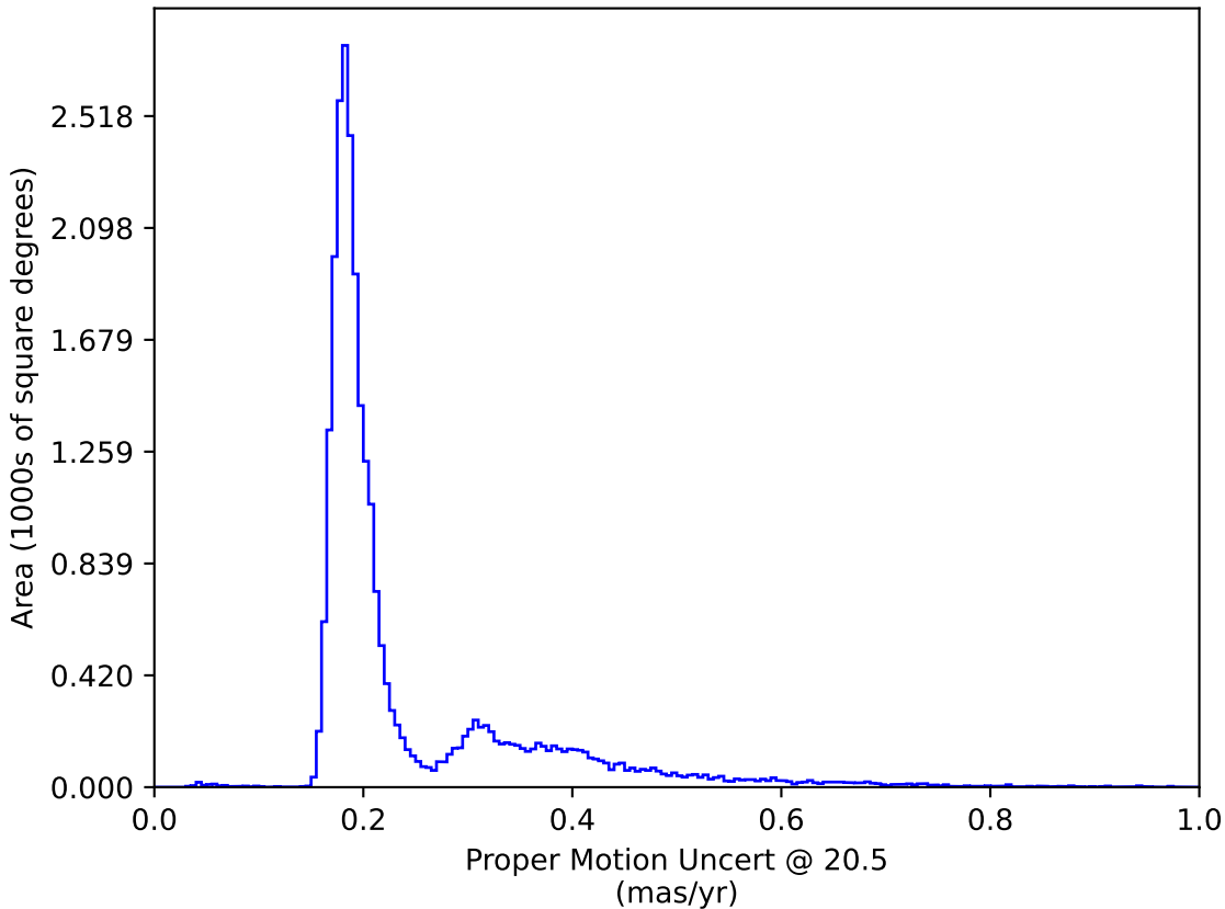
ddf_loaded_half_fl8_v3.3_10yrs : Proper Motion Uncert @ 20.5
