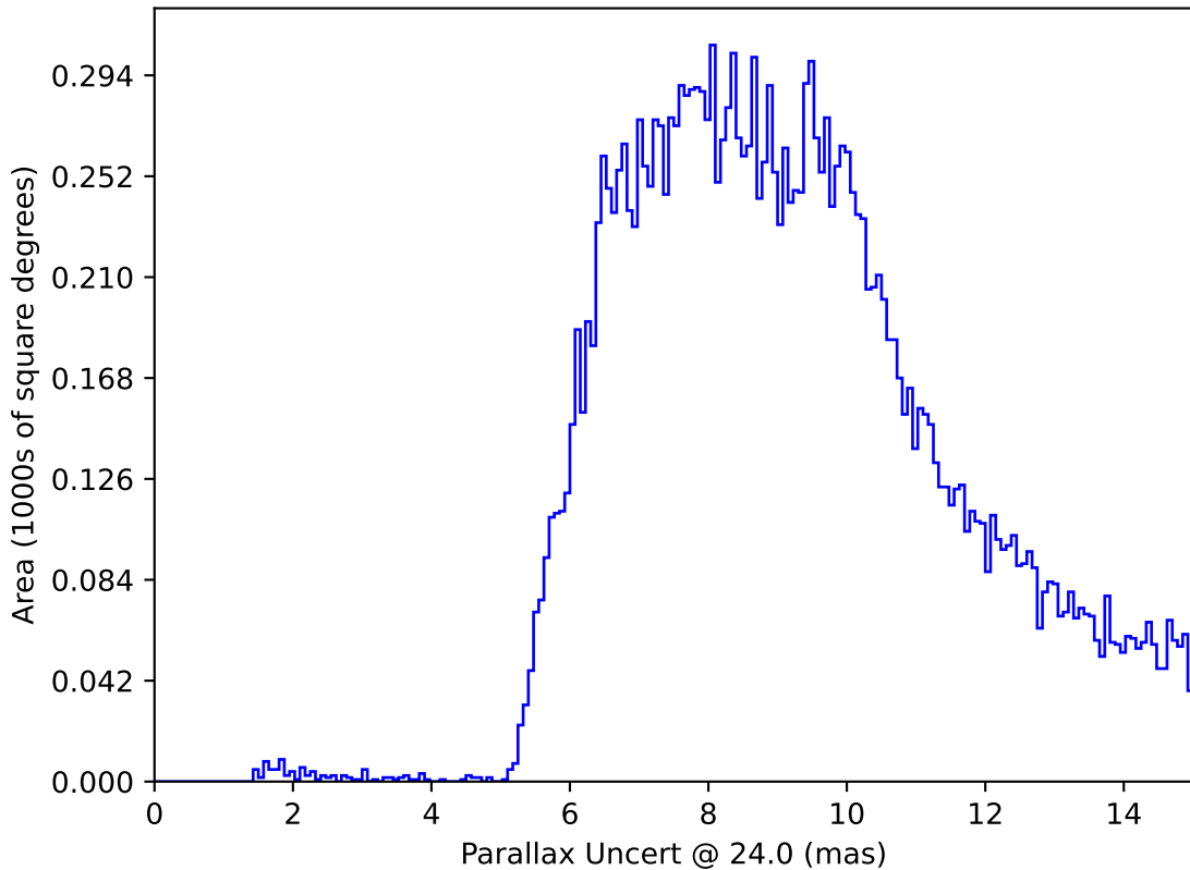
ddf_loaded_half_fl8_v3.3_10yrs : Parallax Uncert @ 24.0
