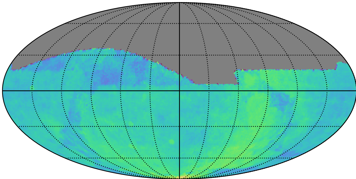
ddf_loaded_half_fl8_v3.3_10yrs : Parallax Coverage @ 24.0
