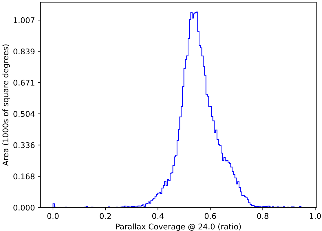
ddf_loaded_half_fl8_v3.3_10yrs : Parallax Coverage @ 24.0
