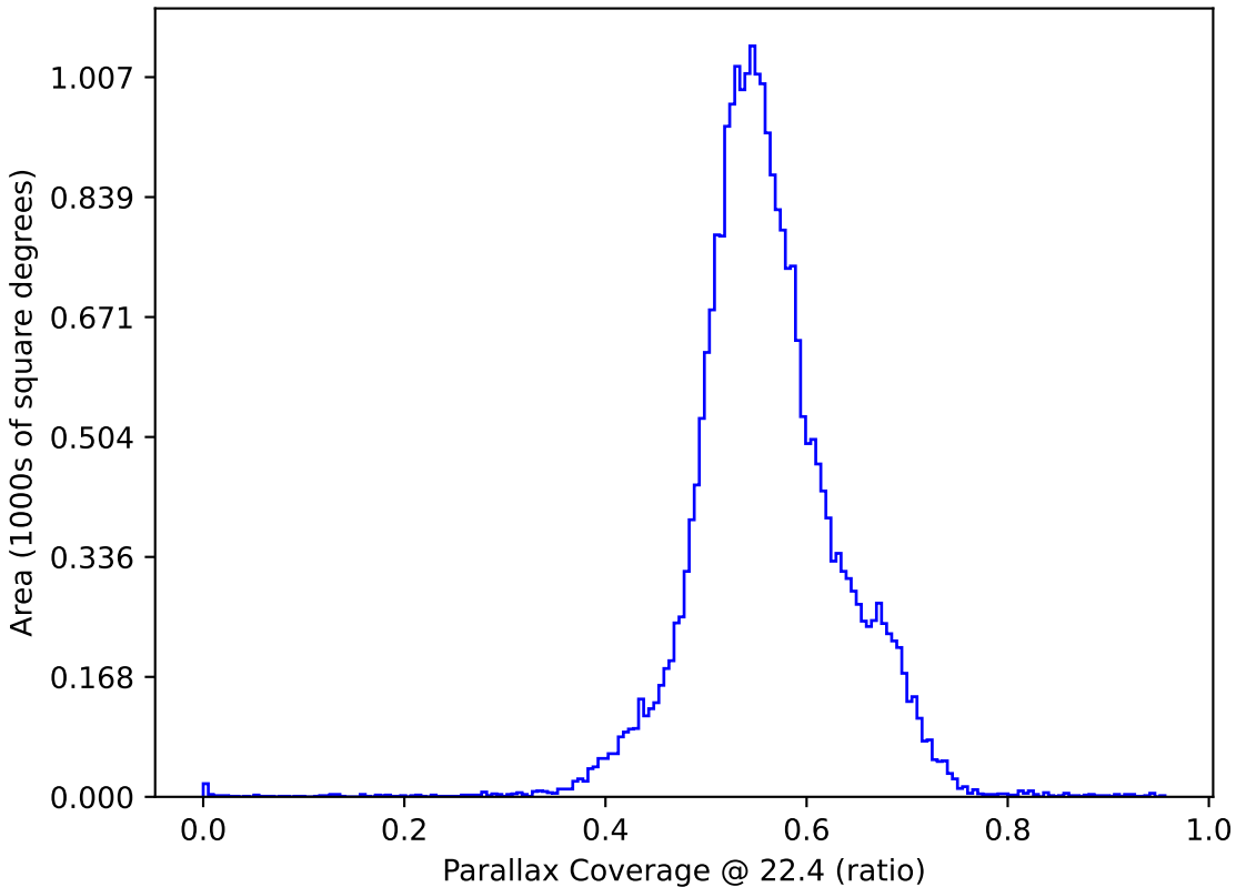
ddf_loaded_half_fl8_v3.3_10yrs : Parallax Coverage @ 22.4
