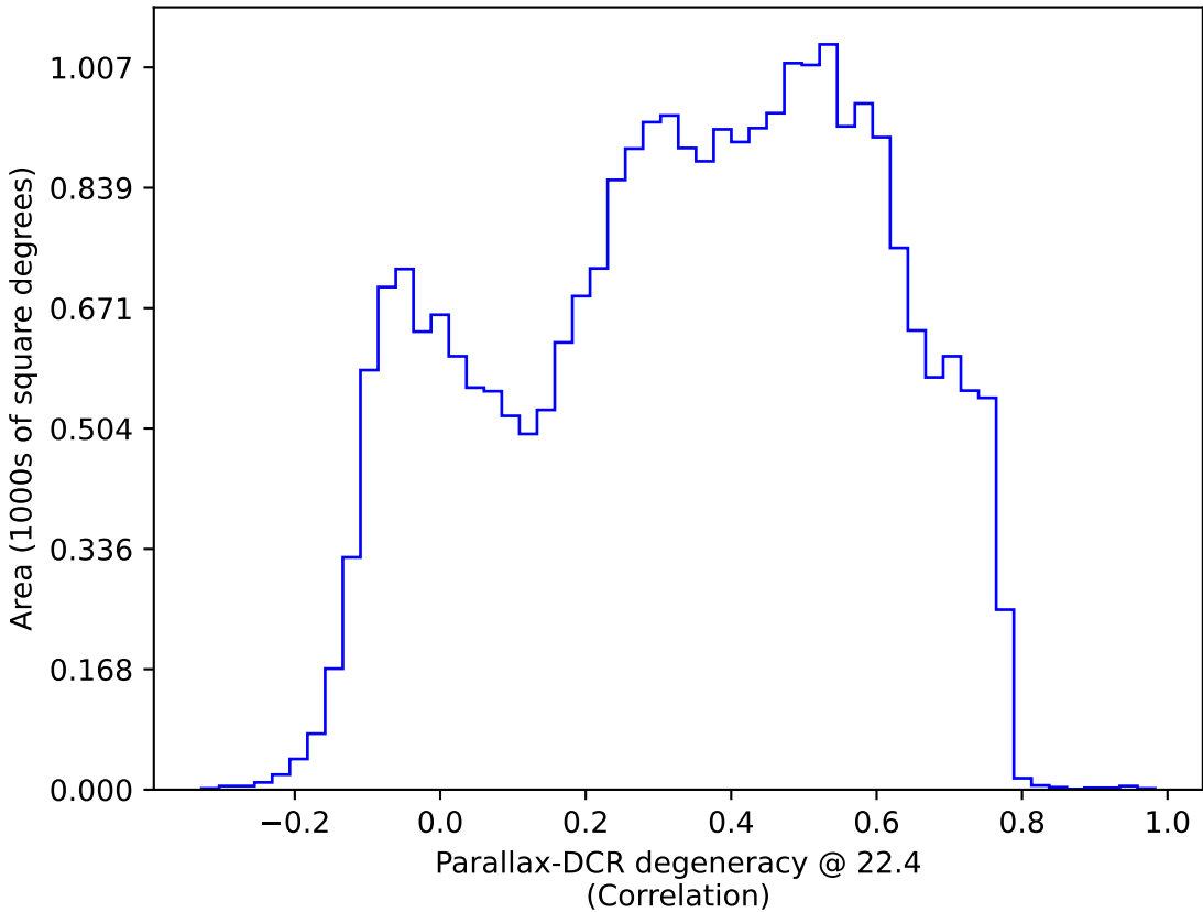
ddf_loaded_half_fl8_v3.3_10yrs : Parallax-DCR degeneracy @ 22.4
