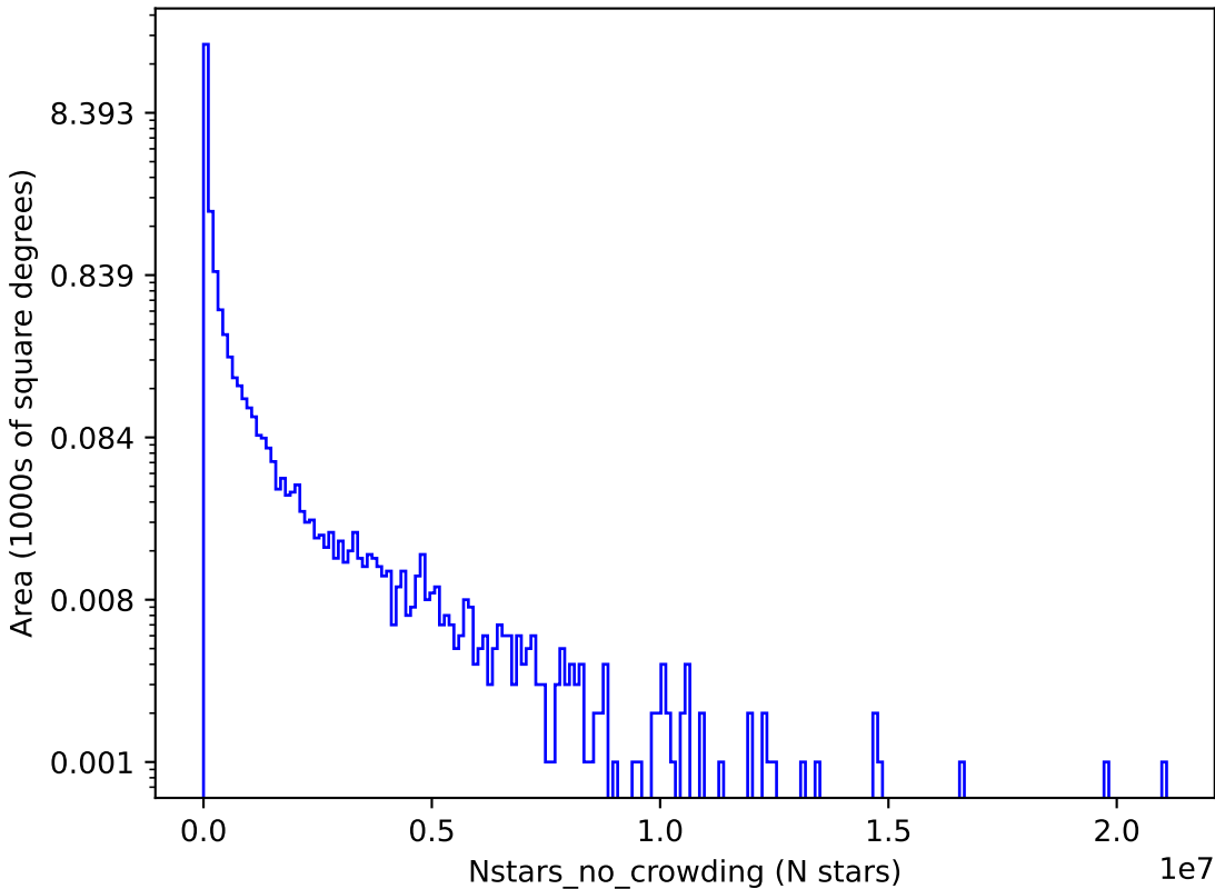
ddf_loaded_half_f18_v3.3_10yrs r: Nstars_no_crowding
