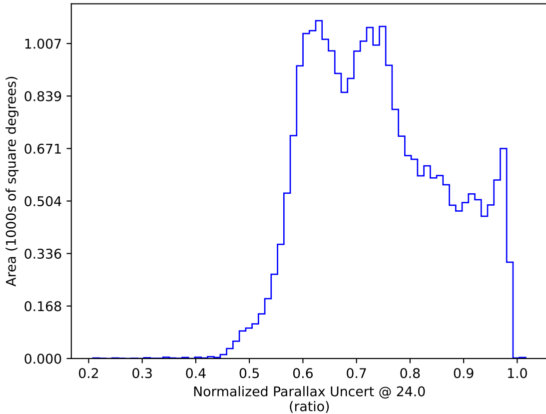
ddf_loaded_half_fl8_v3.3_10yrs : Normalized Parallax Uncert @ 24.0
