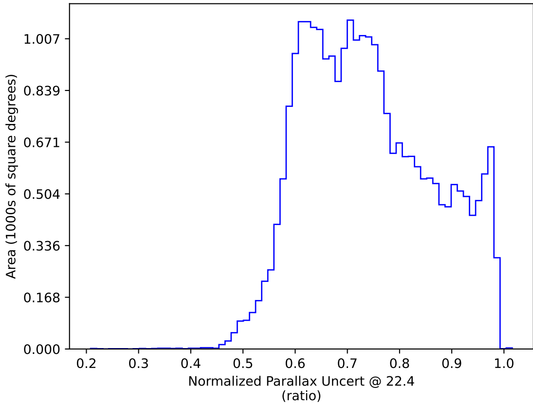
ddf_loaded_half_fl8_v3.3_10yrs : Normalized Parallax Uncert @ 22.4
