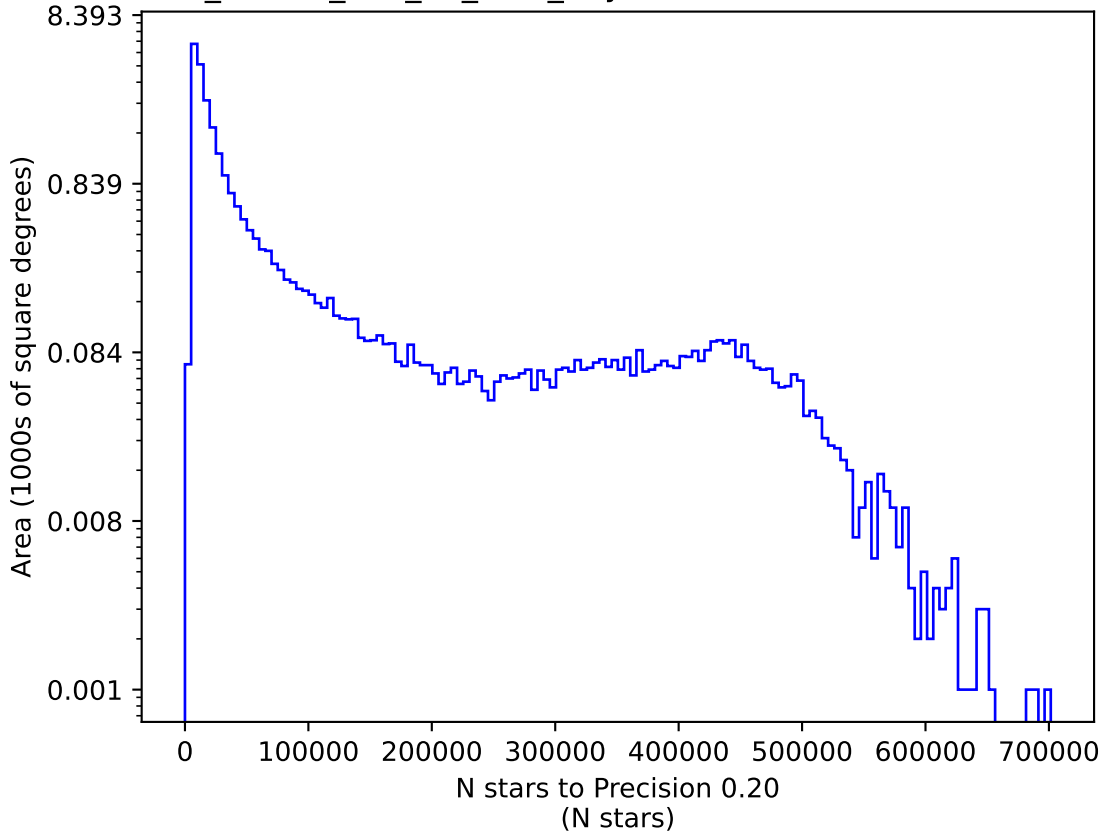
ddf_loaded_half_fl8_v3.3_10yrs i: N stars to Precision 0.20
