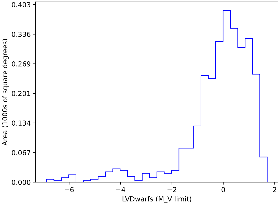
ddf_loaded_half_fl8_v3.3_10yrs gi SCP: LVDwarfs
