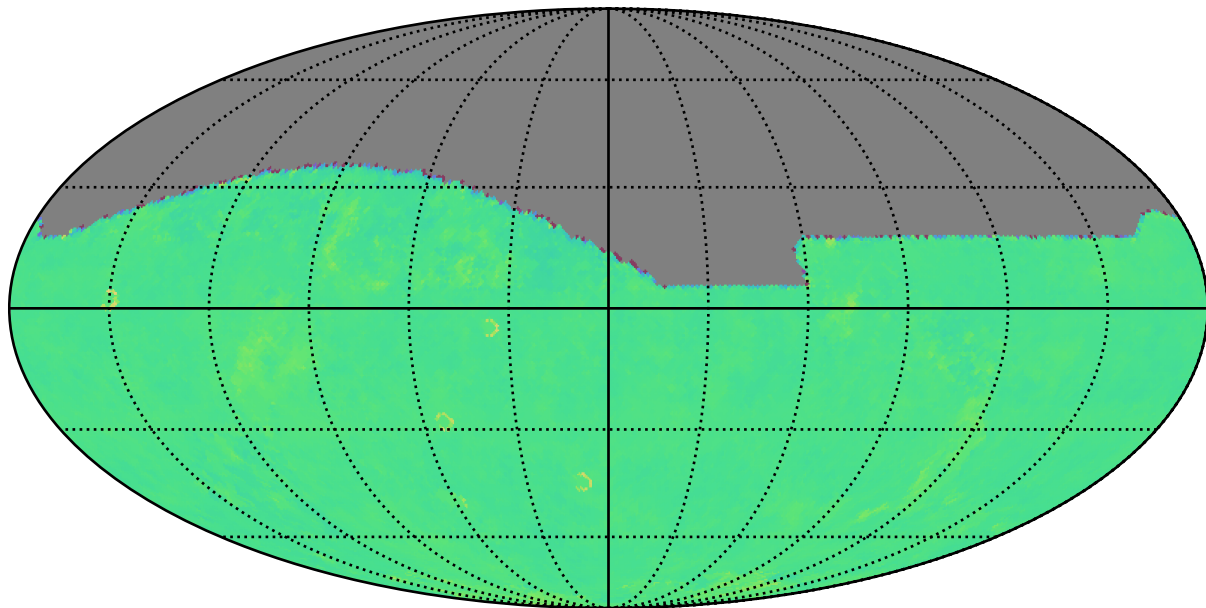
ddf_loaded_half_fl8_v3.3_10yrs z: Kuiper rotTelPos
