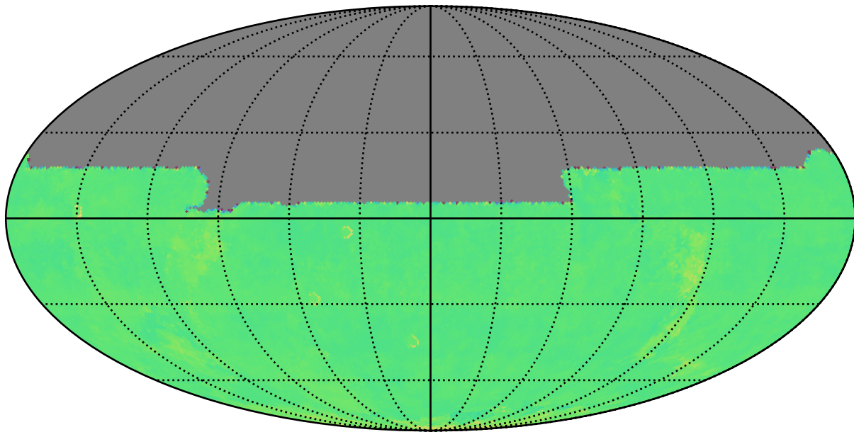
ddf_loaded_half_fl8_v3.3_10yrs y: Kuiper rotTelPos
