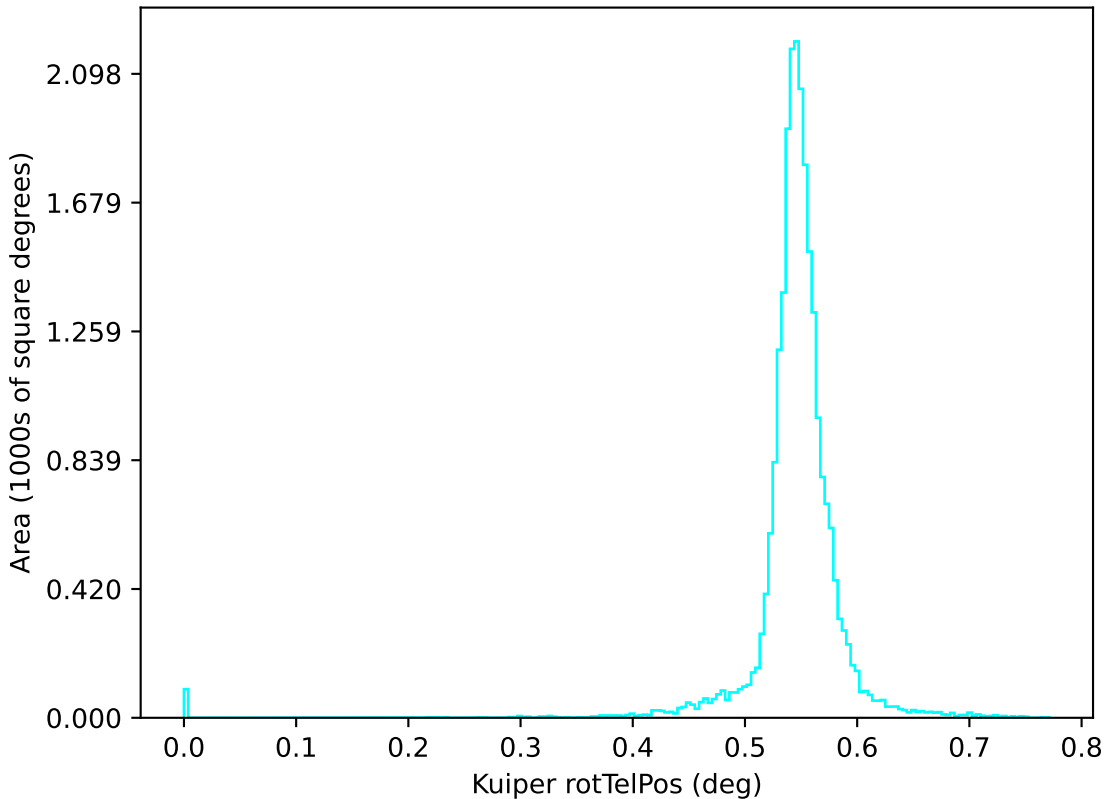
ddf_loaded_half_fl8_v3.3_10yrs u: Kuiper rotTelPos
